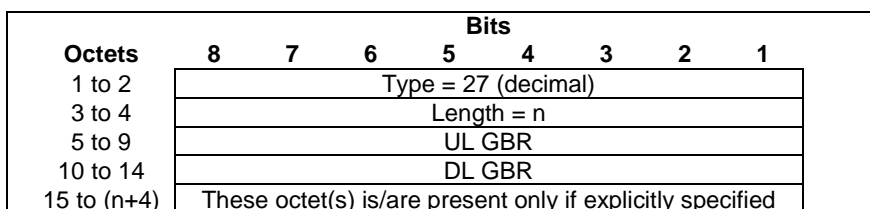
Figure 8.2.9-1: GBR
