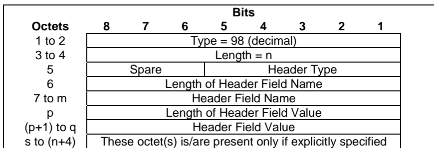
Figure 8.2.67-1: Header Enrichment
