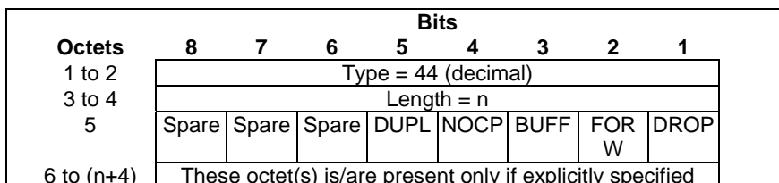
Figure 8.2.26-1: Apply-Action
