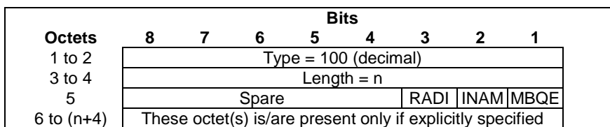
Figure 8.2.68-1: Measurement Information
