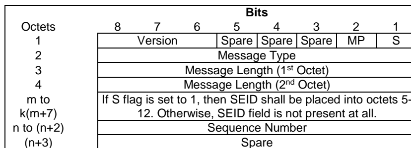
Figure 7.2.2.1-1: General format of PFCP Header
