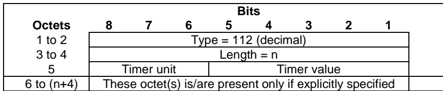
Figure 8.2.78-1: Graceful Release Period
