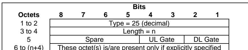
Figure 8.2.7-1: Gate Status
