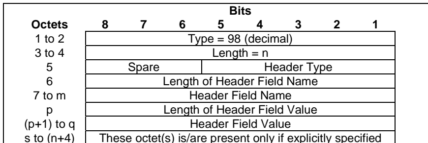
Figure 8.2.67-1: Header Enrichment
