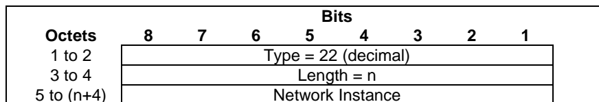
Figure 8.2.4-1: Network Instance
