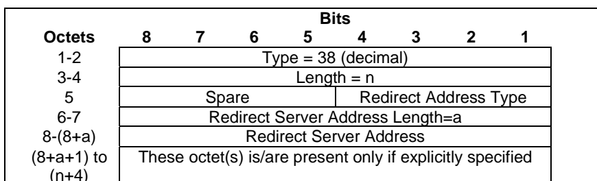
Figure 8.2.20-1: Redirect Information
