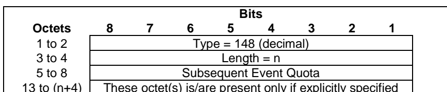
Figure 8.2.112-1: Event Quota
