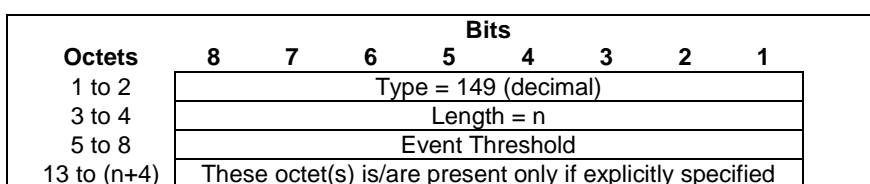
Figure 8.2.113-1: Event Threshold
