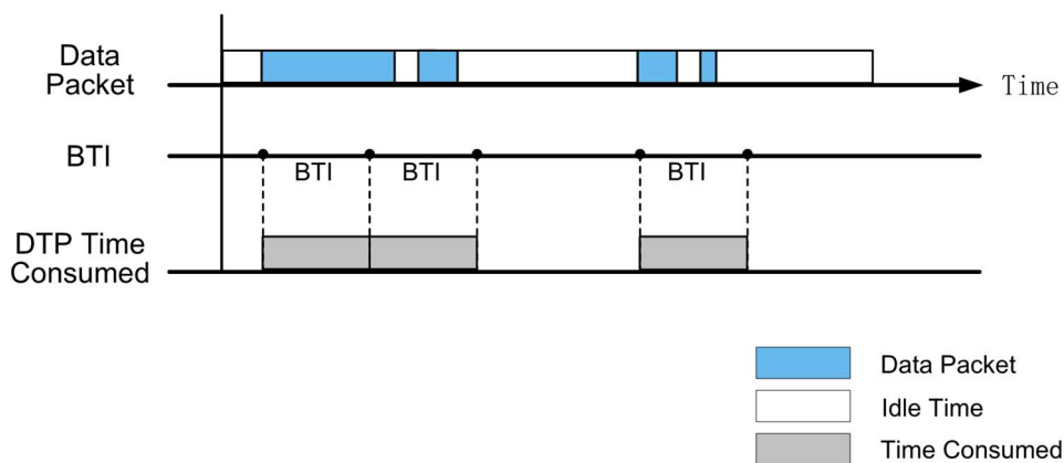
Figure 5.2.2.2-3: DTP based charging
