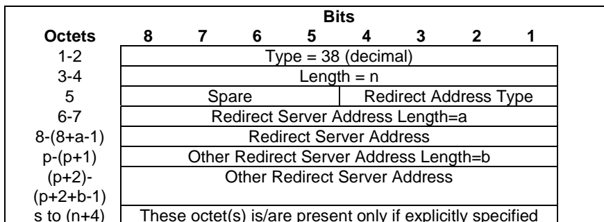
Figure 8.2.20-1: Redirect Information
