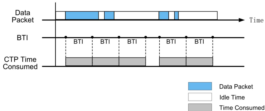
Figure 5.2.2.2-2: CTP based charging
