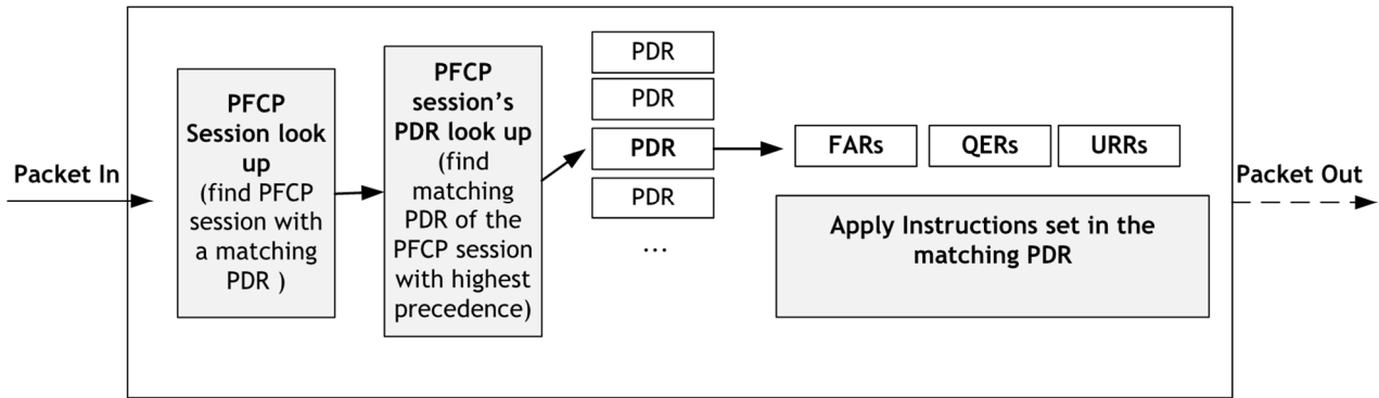
Figure 5.2.1-1: Packet processing flow in the UP function
