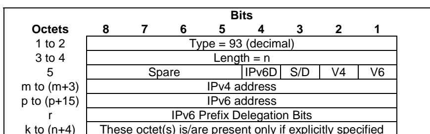
Figure 8.2.62-1: UE IP Address
