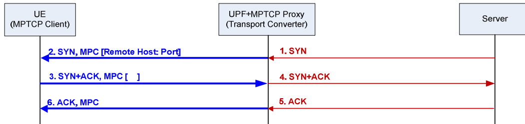
Figure E.2.3-1 –Outgoing Converter-Assisted Multipath TCP Connection Setup
