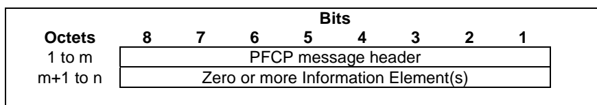
Figure 7.2.1-1: PFCP Message Format
