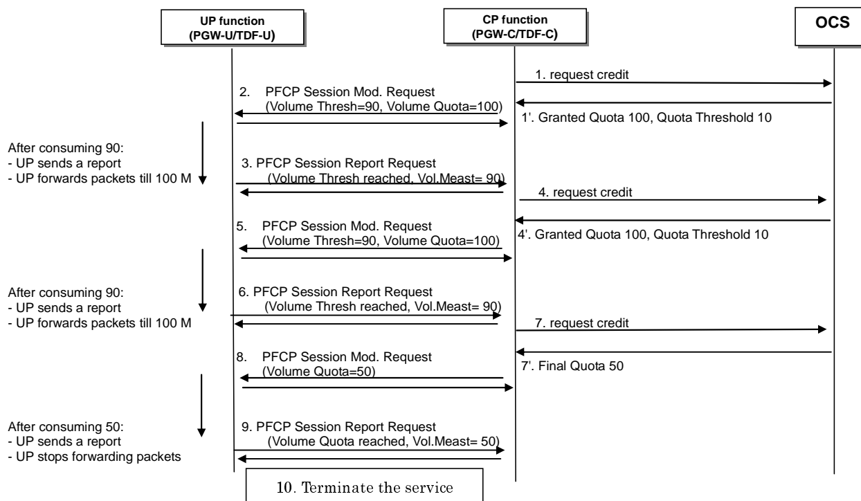
Figure C.2.1.1-1: Online charging with intermediate and final quotas
