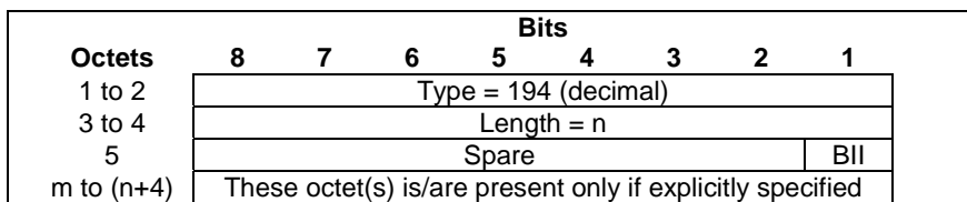
Figure 8.2.140-1: Create Bridge Info for TSC IE
