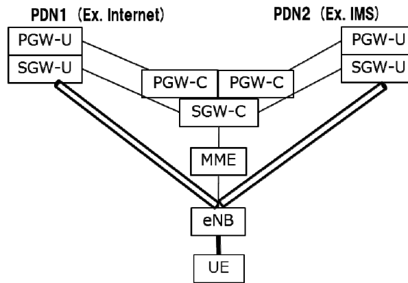
Figure B.2.4 -1: SGW-U/PGW-U colocation with Control and User Plane Separation
