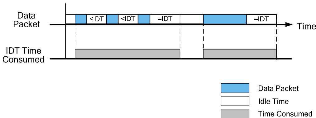
Figure 5.2.2.2-1: IDT based charging
