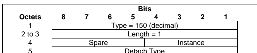
Figure 8.71-1: Detach Type
