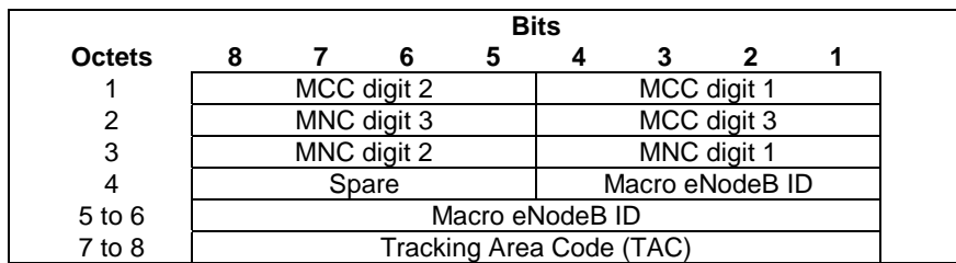
Figure 8.59-2: Source ID for Type eNodeB
