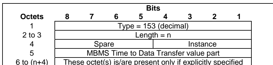
Figure 8.83-1: MBMS Time to Data Transfer
