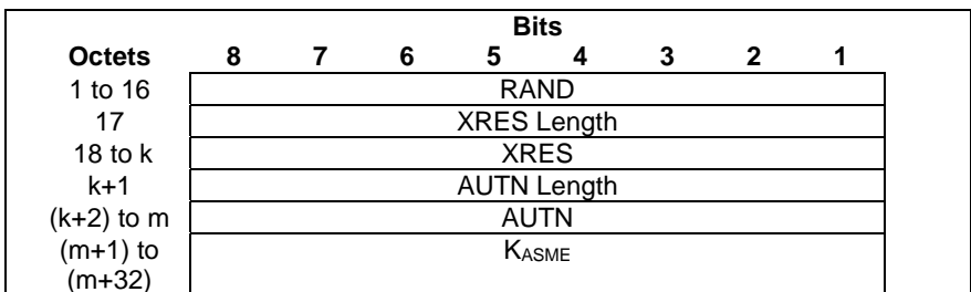
Figure 8.38-9: Authentication Quadruplet
