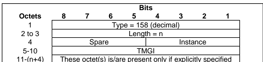
Figure 8.89-1: TMGI
