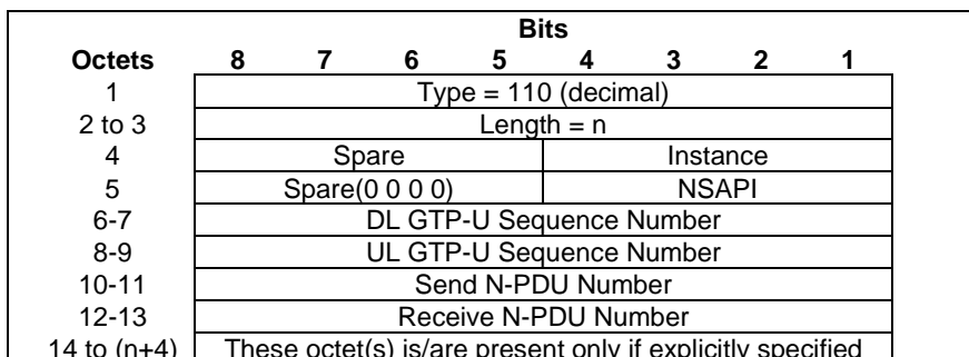
Figure 8.40-1: PDU Numbers
