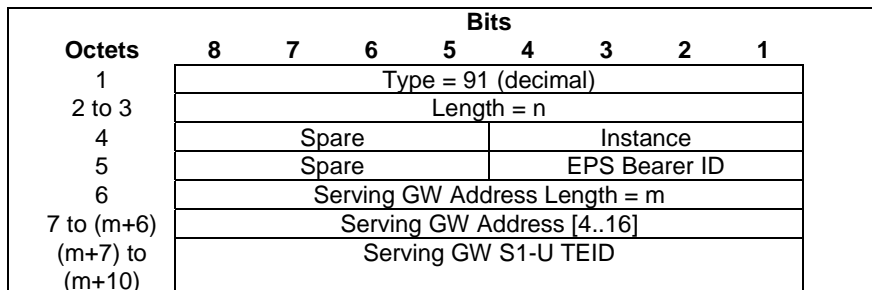
Figure 8.26-1: S1-U Data Forwarding Info
