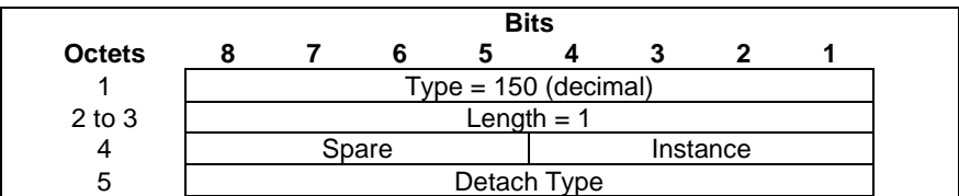
Figure 8.81-1: Detach Type
