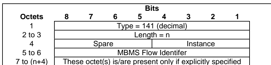
Figure 8.72-1: MBMS Flow Identifier
