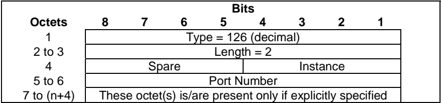
Figure 8.56-1: Port Number
