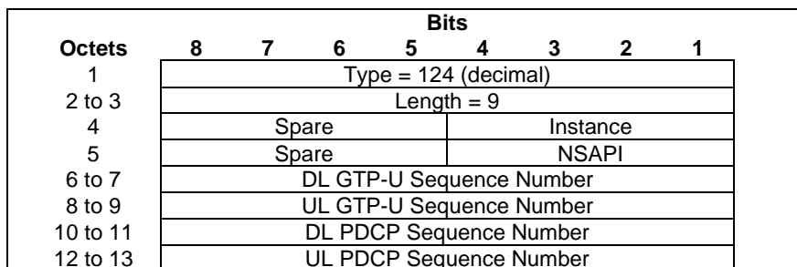
Figure 8.54-1: RAB Context
