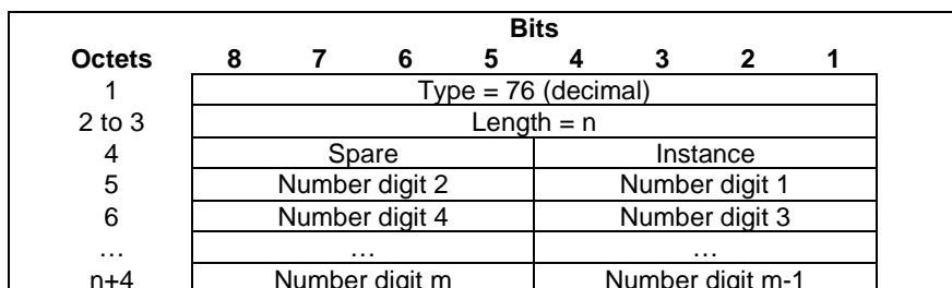
Figure 8.11-1: MSISDN
