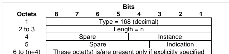
Figure 8.99-1: Action Indication
