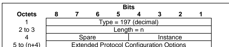
Figure 8.128-1: Extended Protocol Configuration Options (ePCO)
