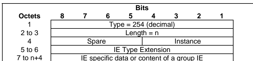
Figure 8.2.1A-1: Information Element with an IE Type Extension field
