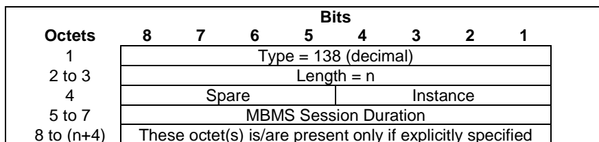
Figure 8.69-1: MBMS Session Duration
