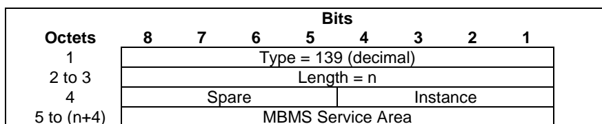
Figure 8.70-1: MBMS Service Area
