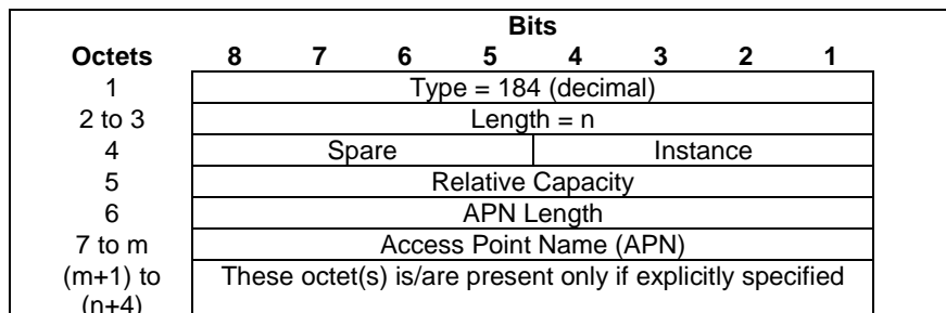
Figure 8.115-1: APN and Relative Capacity
