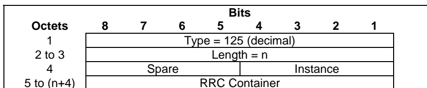
Figure 8.55-1: Source RNC PDCP context info
