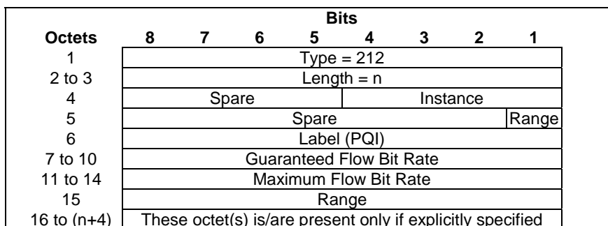
Figure 8.143-1: PC5 QoS Flow
