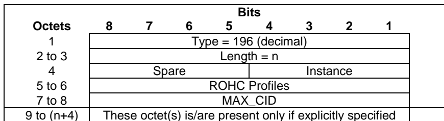
Figure 8.127-1: Header Compression Configuration
