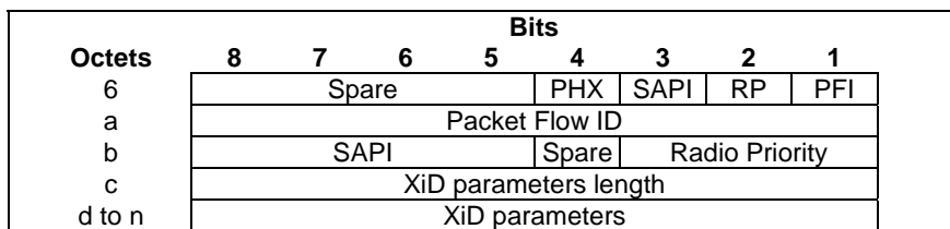
Figure 8.48-3: BSS Container
