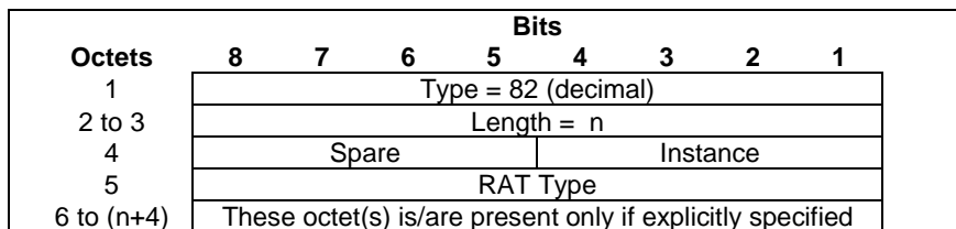
Figure 8.17-1: RAT Type
