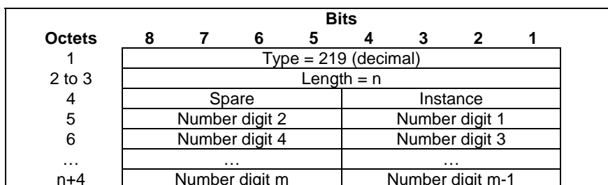
Figure 8.150-1: Alternative IMSI
