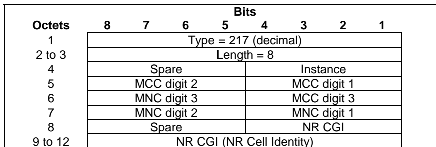
Figure 8.148-1: PSCell ID
