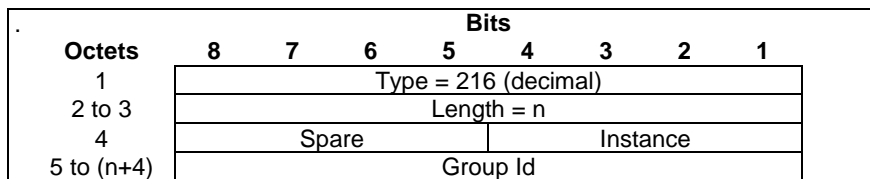
Figure 8.147-1: Group Id
