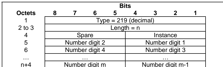
Figure 8.150-1: Alternative IMSI
