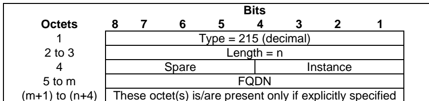
Figure 8.146-1: PGW FQDN
