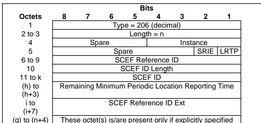
Figure 8.137-1: Monitoring Event Extension Information
