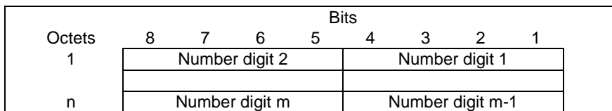
Figure 12.1.1.14-1: Unauthenticated IMSI
