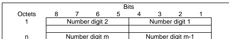
Figure 12.1.1.14-1: Unauthenticated IMSI
