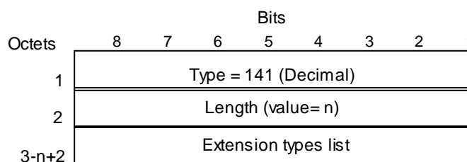
Figure 8.5-1: Extension Header Type List Information Element
