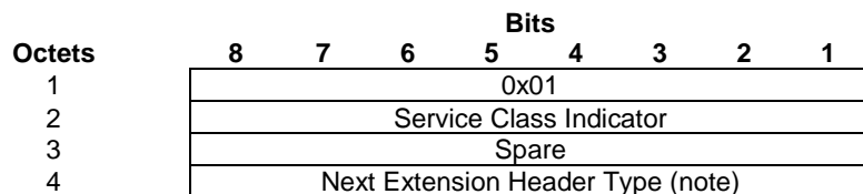
Figure 5.2.2.3-1: Service Class Indicator Extension Header
