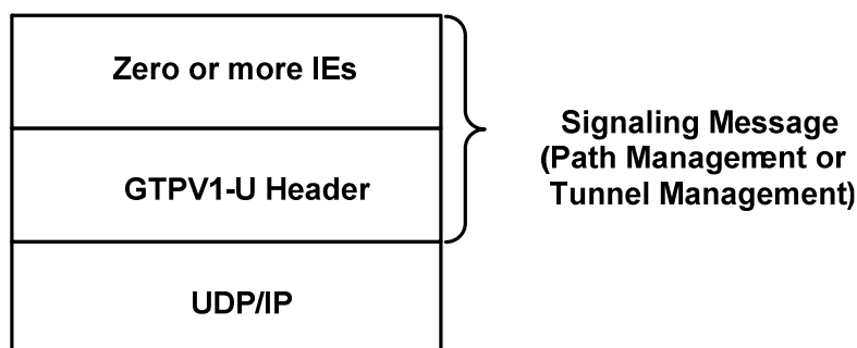
Figure: 4.4-2 Signaling Message Protocol Stack
