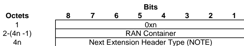
Figure 5.2.2.4-1: RAN Container Extension Header
