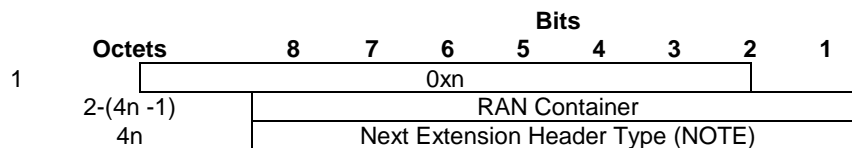
Figure 5.2.2.4-1: RAN Container Extension Header
