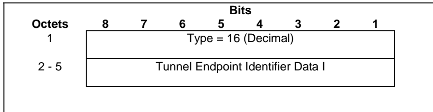
Figure 8.3-1: Tunnel Endpoint Identifier Data I Information Element
