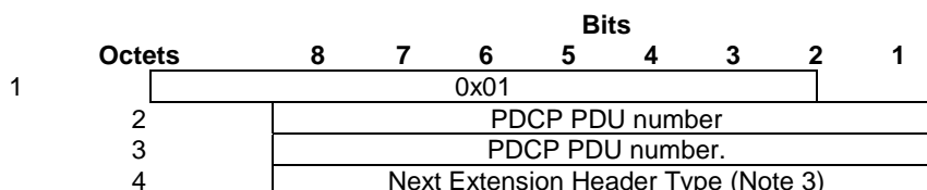
Figure 5.2.2.2-1: PDCP PDU Number Extension Header
