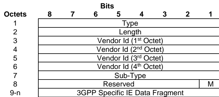
Figure 4.2-1: 3GPP Mobile IPv6 Option
