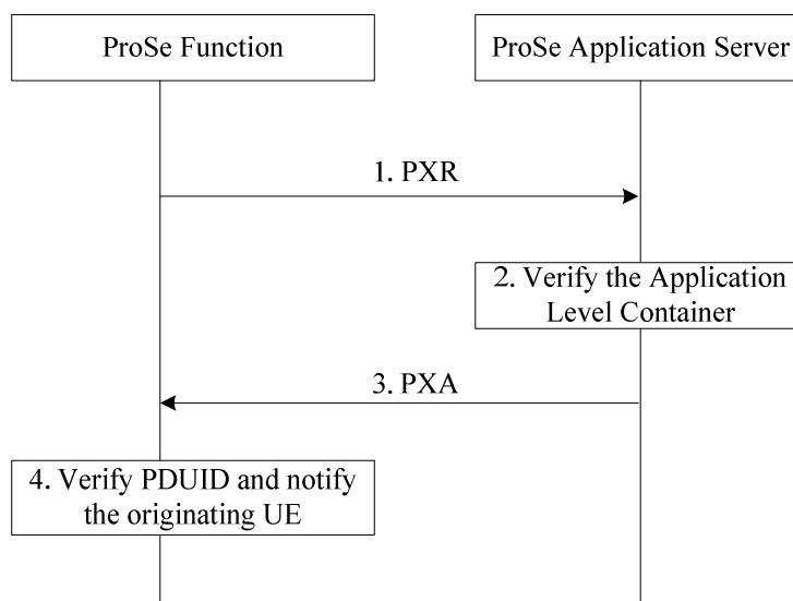
Figure A.2.4: Authorization for Monitor request with application-controlled extension procedure
