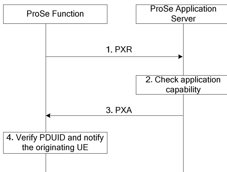
Figure A.2.2: Authorization for announce request with application-controlled extension procedure
