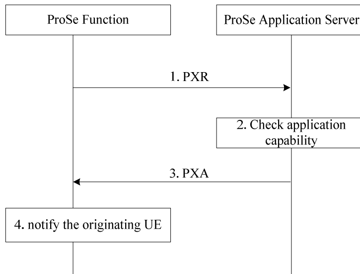
Figure A.2.11: Authorization for open discovery announce request with application-controlled extension procedure
