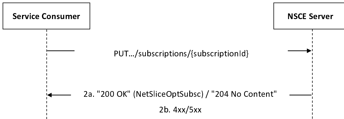
Figure 5.5.2.2.3-1: Procedure for Network Slice Optimization Subscription Update
