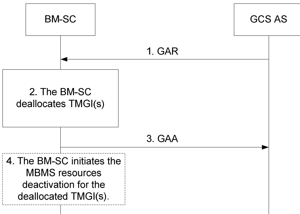
Figure A.1.2-1: TMGI Deallocation Procedure
