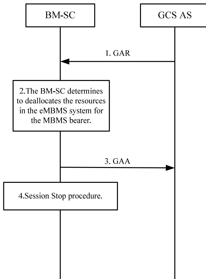
Figure A.2.2.1: Deactivate MBMS bearer Procedure
