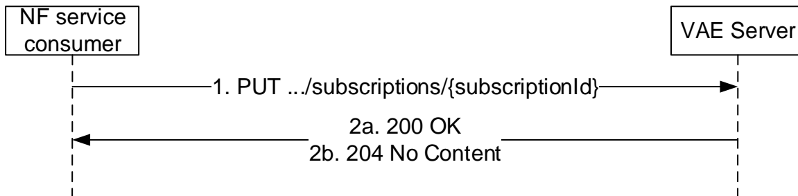
Figure 5.8.2.4.2-1: Update Session
