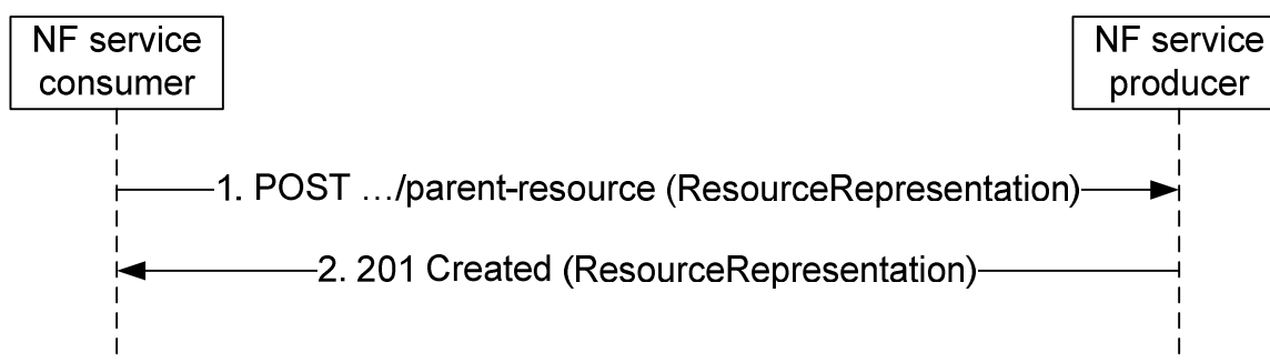
Figure 4.6.1.1.1.2-1: Creating a resource using POST
