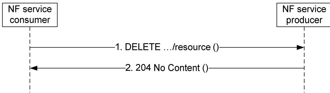
Figure 4.6.1.1.4-1: Deleting a resource
