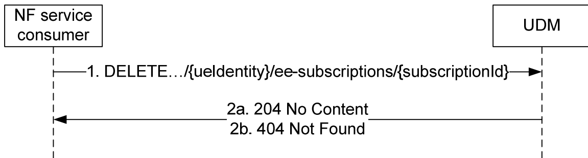
Figure 5.2.2.3.2-1: NF service consumer unsubscribes to notifications
