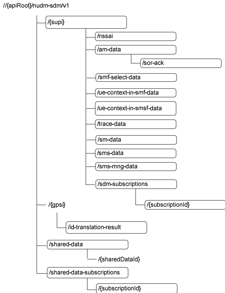
Figure 6.1.3.1-1: Resource URI structure of the nudm-sdm API
