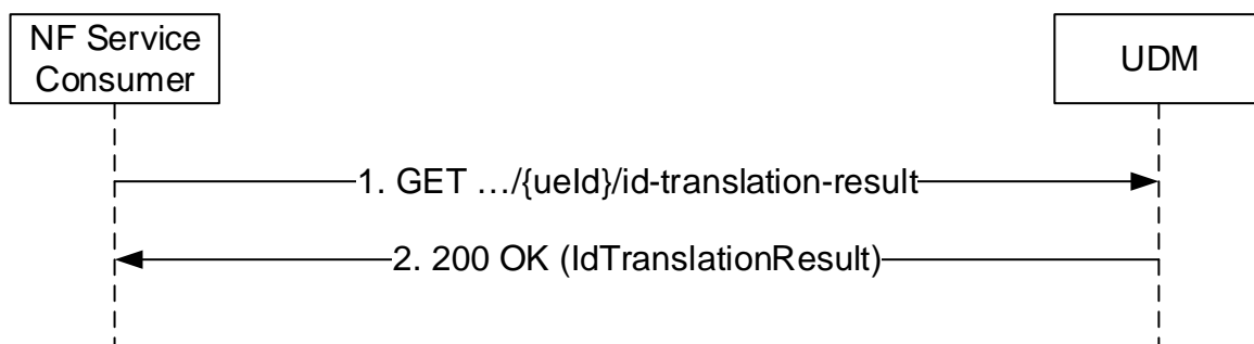
Figure 5.2.2.2.10-1: Identifier Translation
