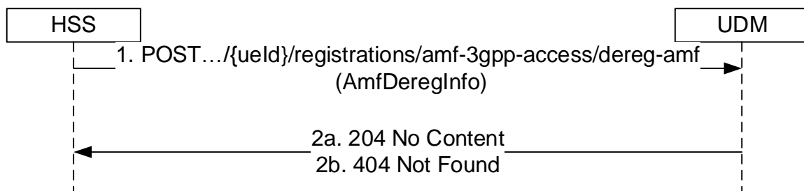
Figure 5.3.2.9.2-1: AMF-Deregistration
