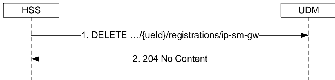
Figure 5.3.2.4.7-1: IP-SM-GW deregistration
