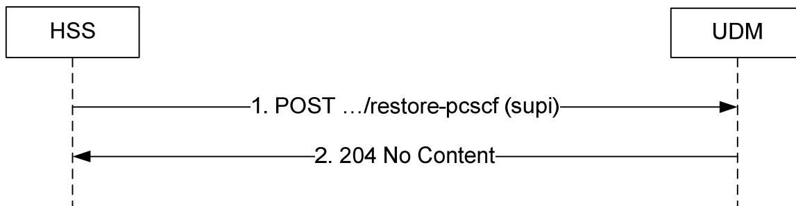
Figure 5.3.2.8.2-1: P-CSCF-RestorationTrigger
