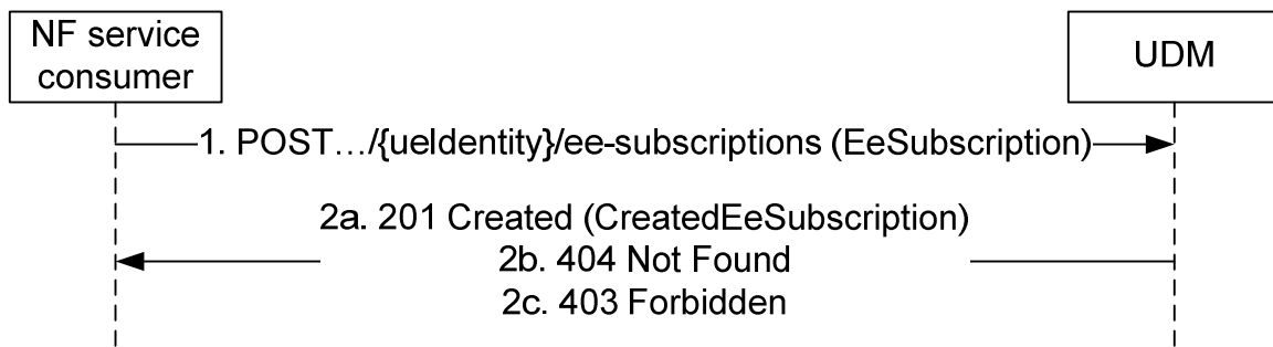
Figure 5.5.2.2-1: NF service consumer subscribes to notifications
