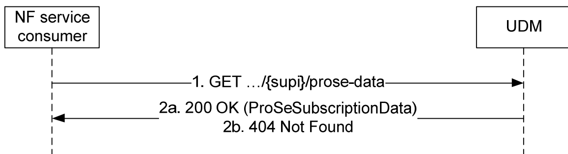
Figure 5.2.2.2.22-1: Requesting a UE's ProSe Subscription Data
