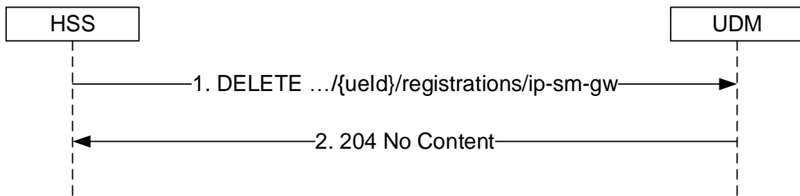
Figure 5.3.2.4.7-1: IP-SM-GW deregistration
