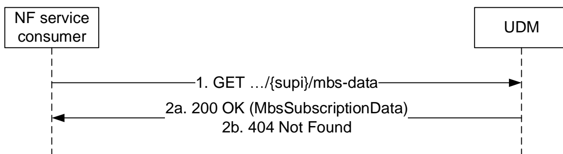
Figure 5.2.2.2.23-1: Requesting a UE's 5MBS Subscription Data
