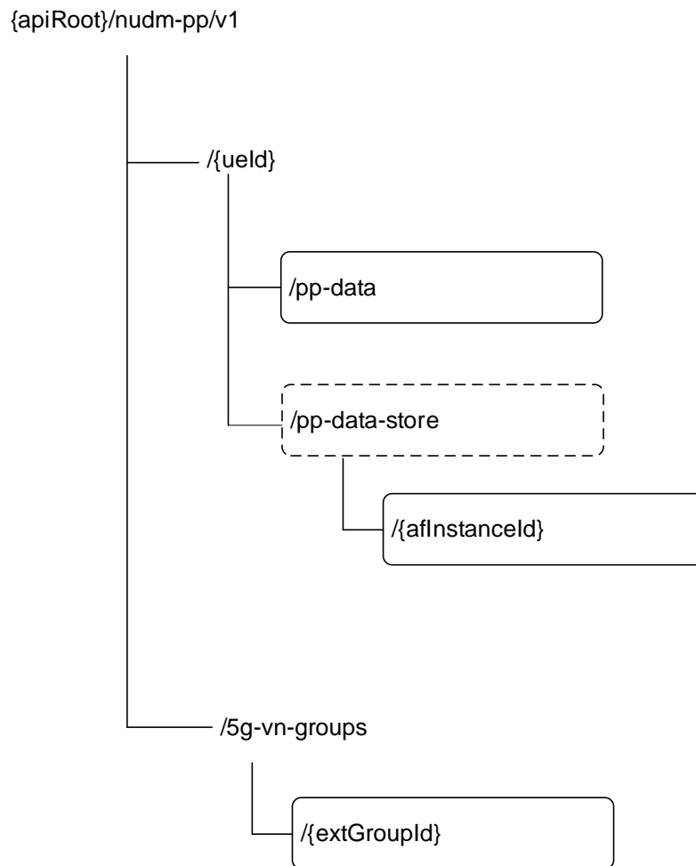
Figure 6.5.3.1-1: Resource URI structure of the Nudm_PP API
