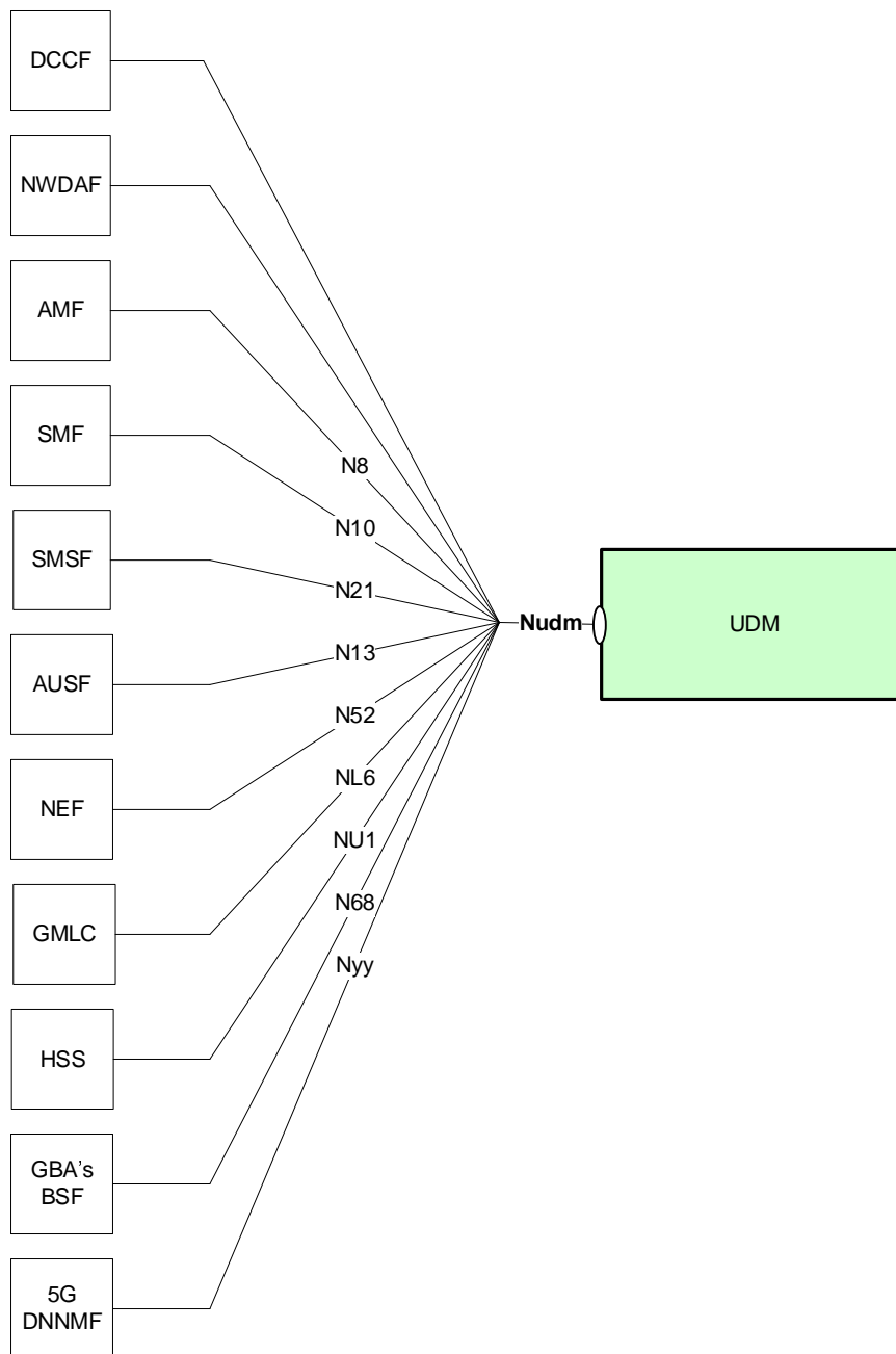
Figure 4.1-1: Reference model – UDM
