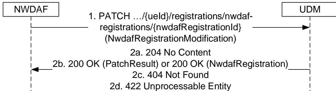
Figure 5.3.2.6.4-1: NWDAF registration parameter update
