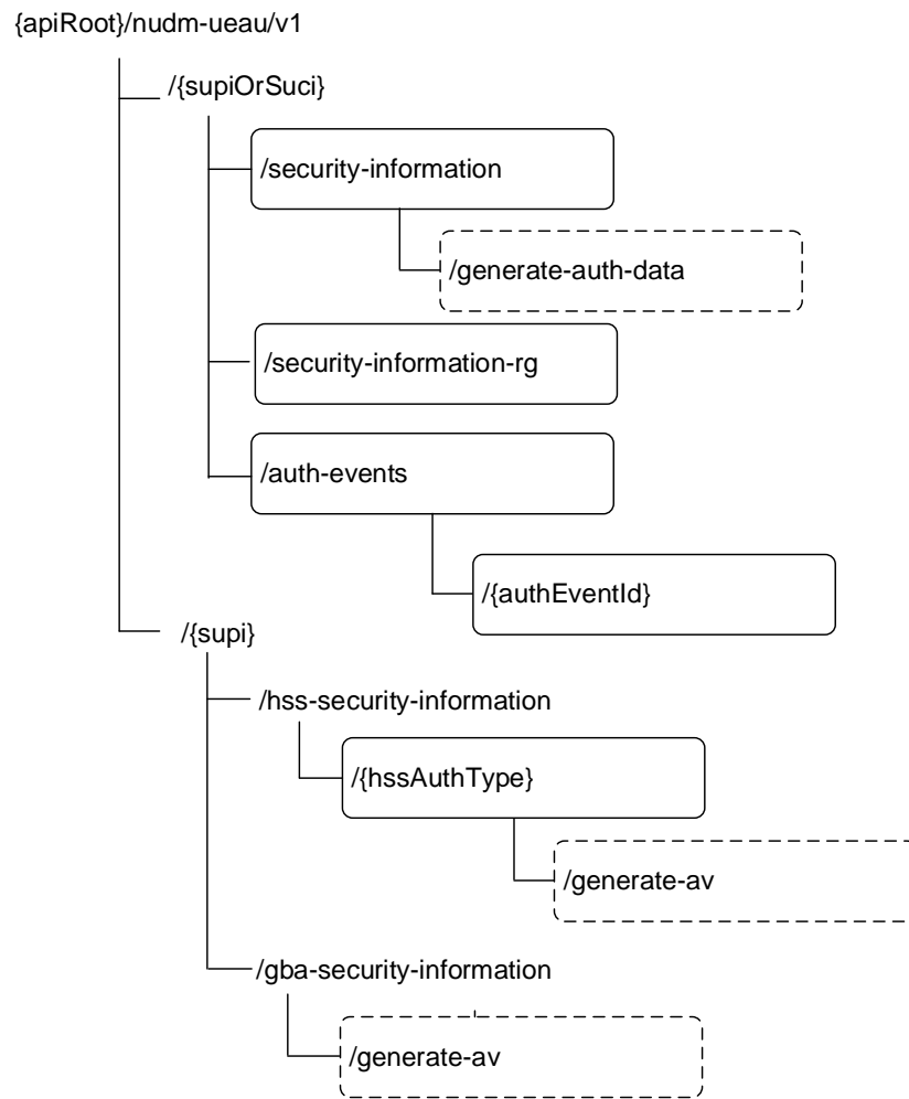
Figure 6.3.3.1-1: Resource URI structure of the Nudm_UEAU API
