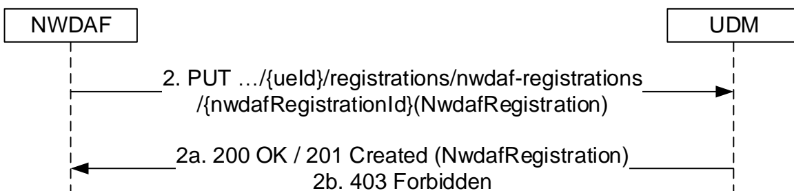
Figure 5.3.2.2.8-1: NWDAF registration
