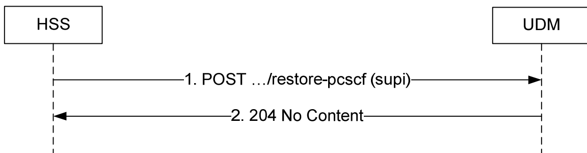
Figure 5.3.2.8.2-1: P-CSCF-RestorationTrigger
