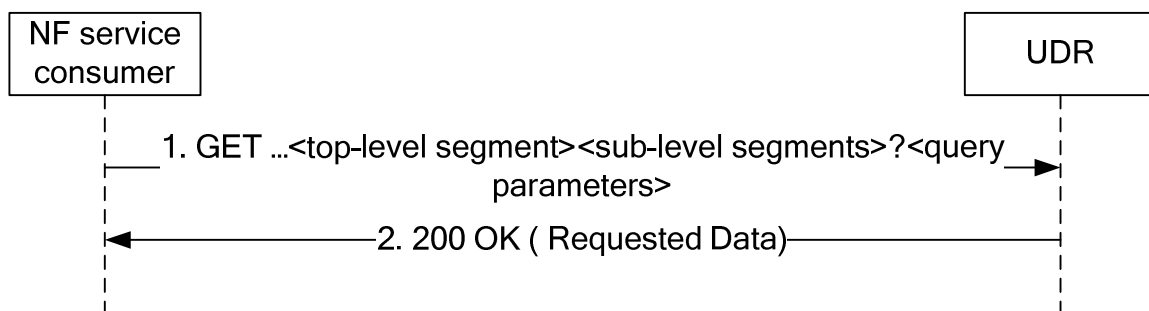
Figure 5.2.2.2.2-1: Retrieving Data
