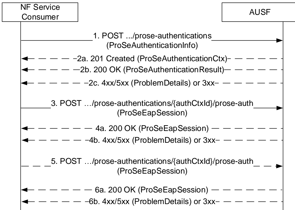
Figure 5.2.2.4.1-1: ProSe Authentication
